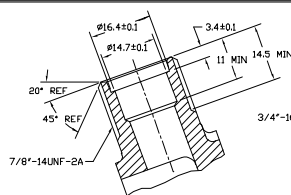
SECTION E-E
