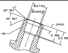
SECTION F-F
