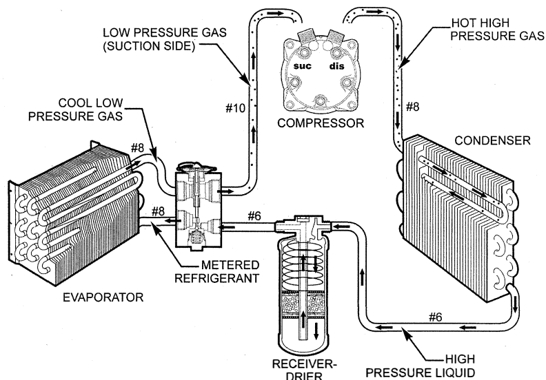
TYPICAL REFRIGERANT FLOW PATTERN
